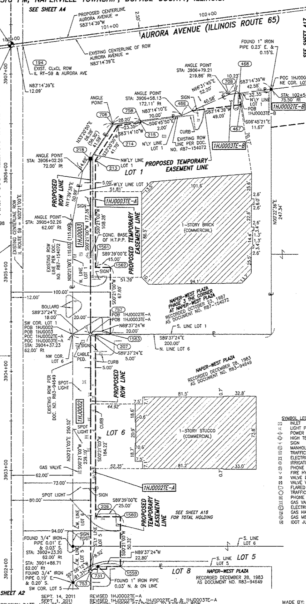
PROJECT COORDINATES ARE SHOWN COORDINATE TABLE ~ EAST NEW YORK ST./AURORA AVE.
