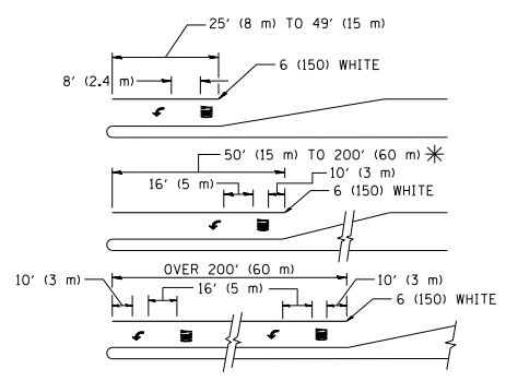
TYPICAL LEFT (OR RIGHT) TURN LANE TYPICAL TURN LANE MARKING
