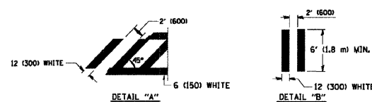
TYPICAL CROSSWALK MARKING
