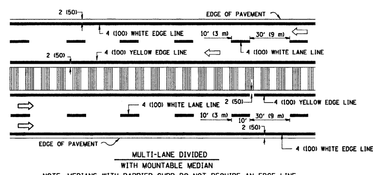
TYPICAL LANE AND EDGE LINE MARKING NOTE: MEDIANS WITH BARRIER CURB DO NOT REQUIRE AN EDGE LINE
