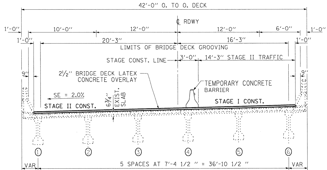
PROPOSED CROSS SECTION LOOKING AHEAD
