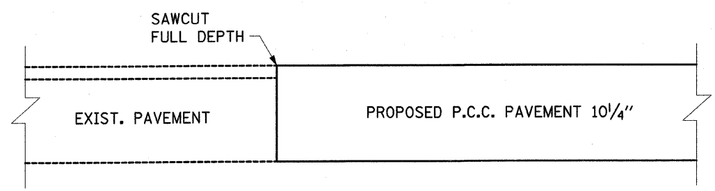
TRANSITION AT STA 1325+65
