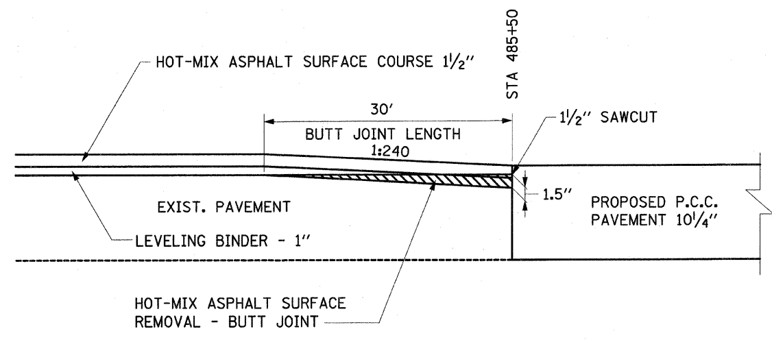
TRANSITION AT STA 485+50
