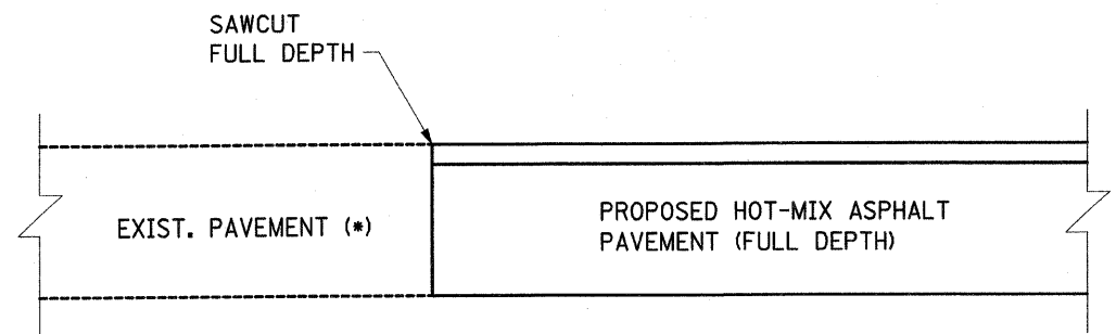
TRANSITION DETAIL
