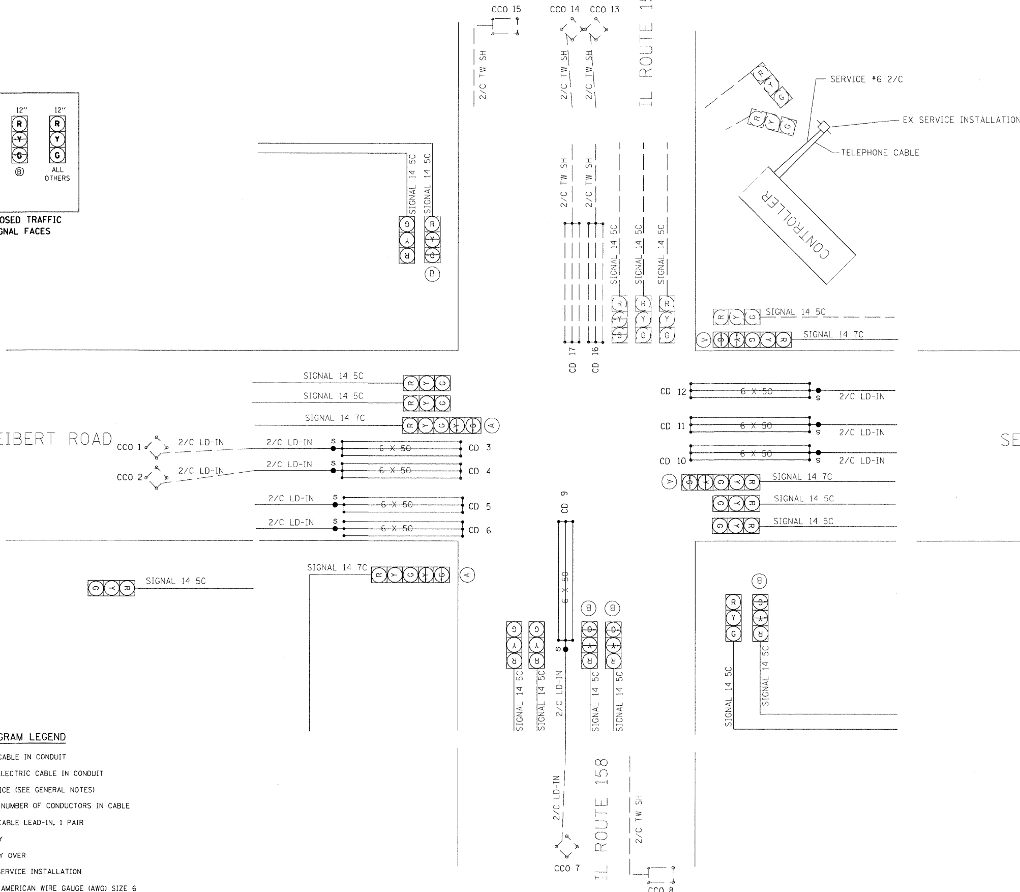
CABLE DIAGRAM
