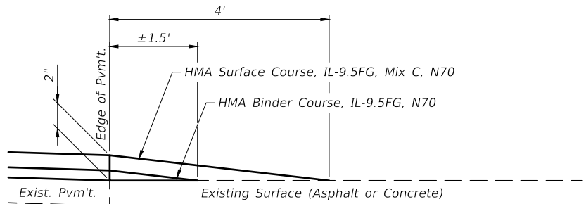
SECTION A-A PRIVATE ENTRANCE - ASPHALT (Est. No. = 3)
