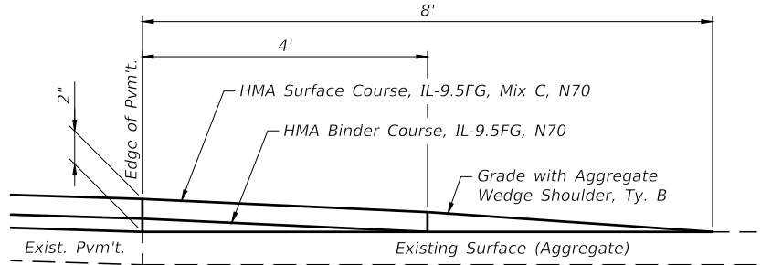
SECTION A-A PRIVATE ENTRANCE - AGGREGATE (Est. No. = 19)
