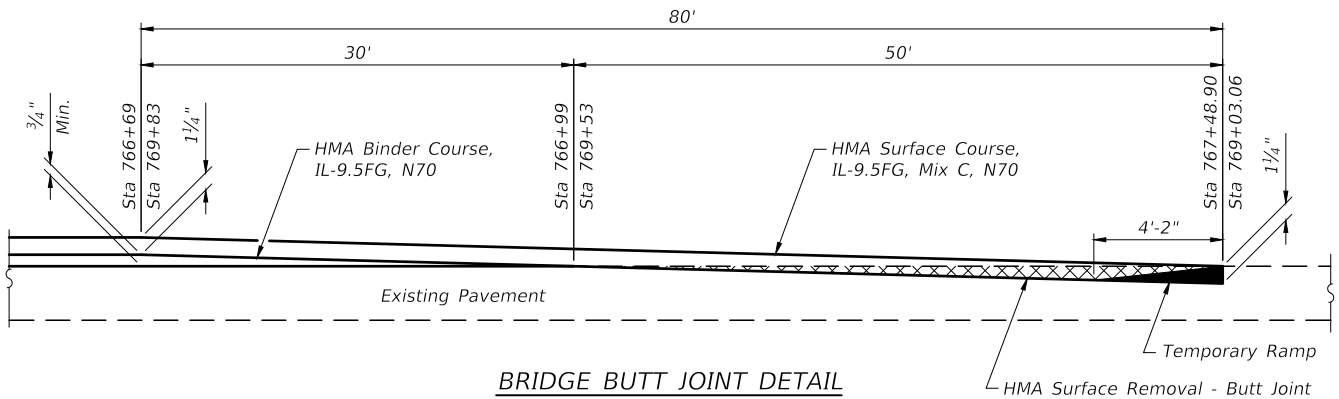
BEGINNING & ENDING BUTT JOINT DETAIL
