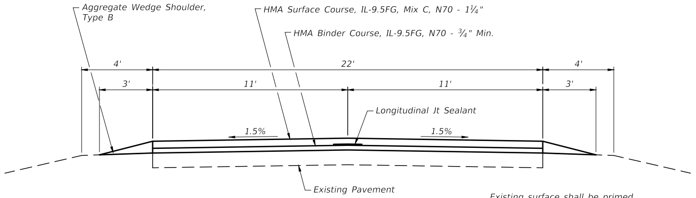
TYPICAL SECTION
