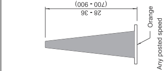
TYPE I BARRIER
