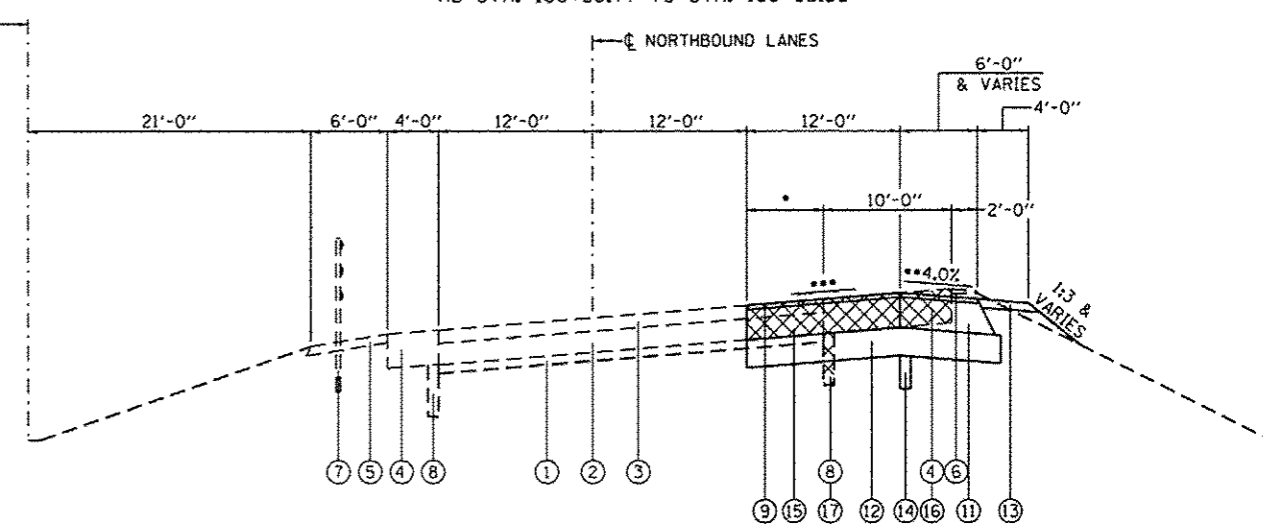
TYPICAL SECTION 2
