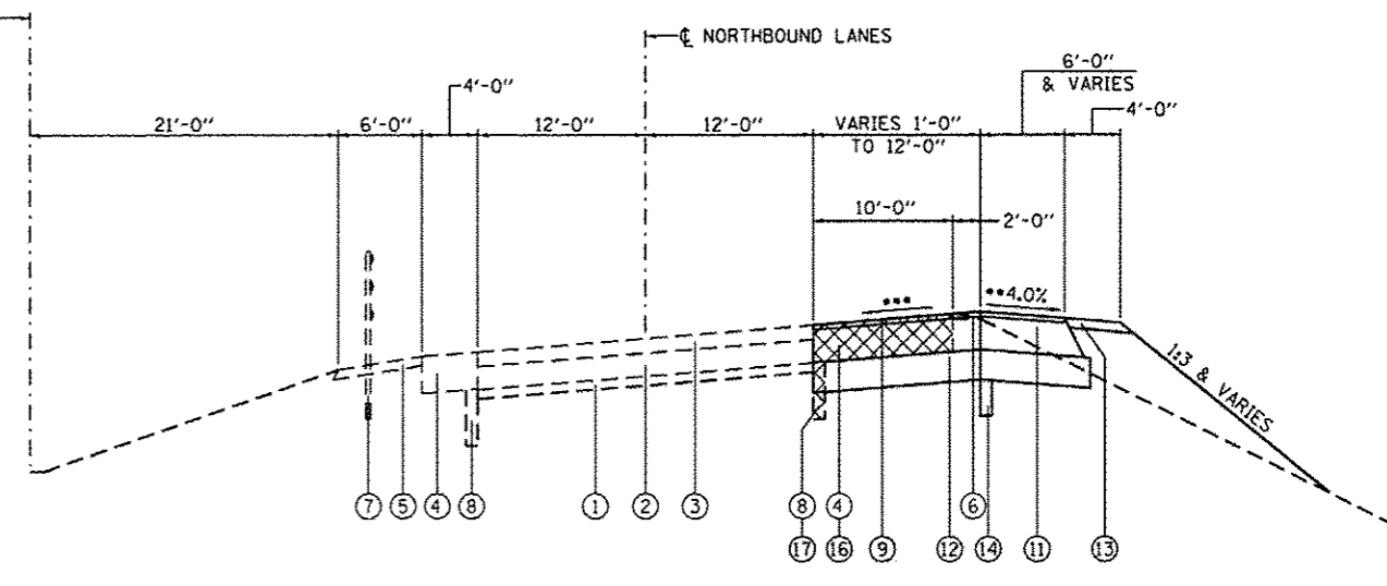
TYPICAL SECTION 2
