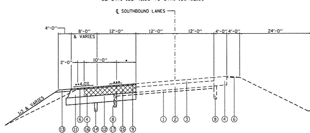
TYPICAL SECTION 1
