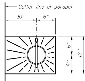
TOP PLAN
