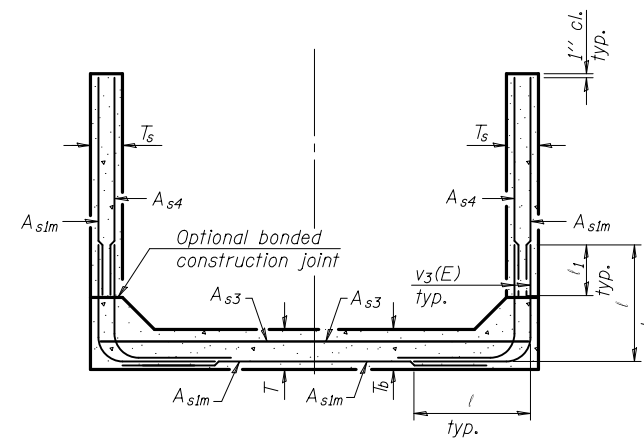
ALTERNATE SECTION D-D
