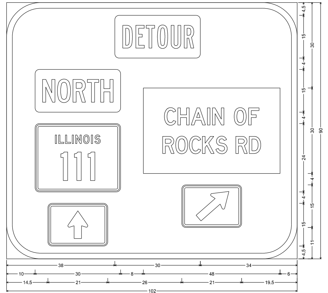
12.0" Radius, 2.0" Border, Black on Orange; M4-8; M3-1; M6-3; COR-W; M6-2R;
