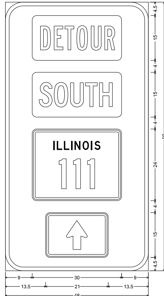
6.0" Radius, 1.3" Border, Black on Orange; M4-8; M3-3; M6-3;
