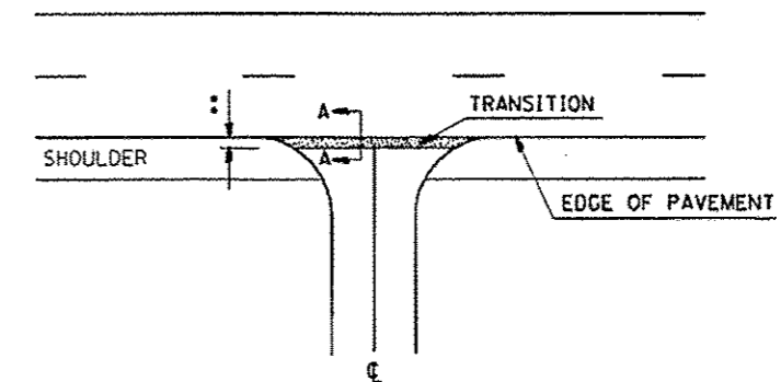
SIDEROAD DETAIL
