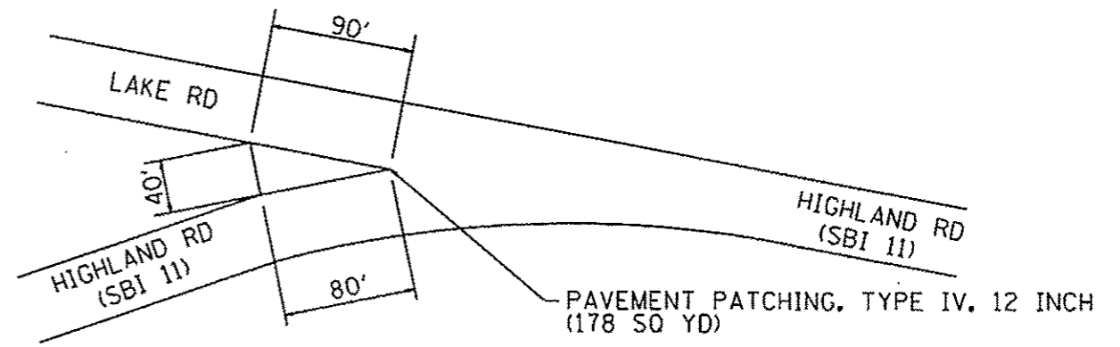
PAVEMENT PATCHING DETAIL
