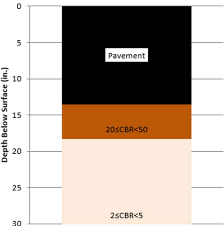
CBR vs. Depth Below Surface (in.) Location #3 - CH 25
