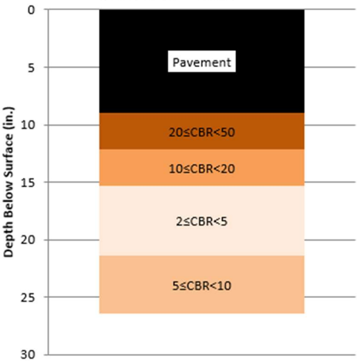
CBR vs. Depth Below Surface (in.) Location #6 - CH 25
