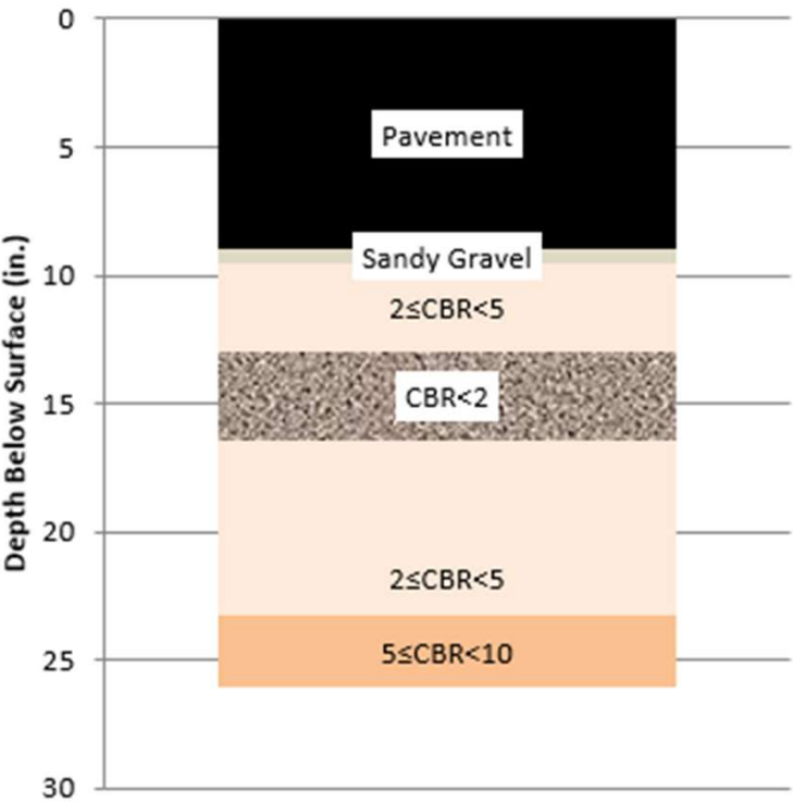
CBR vs. Depth Below Surface (in.) Location #9 - CH 25
