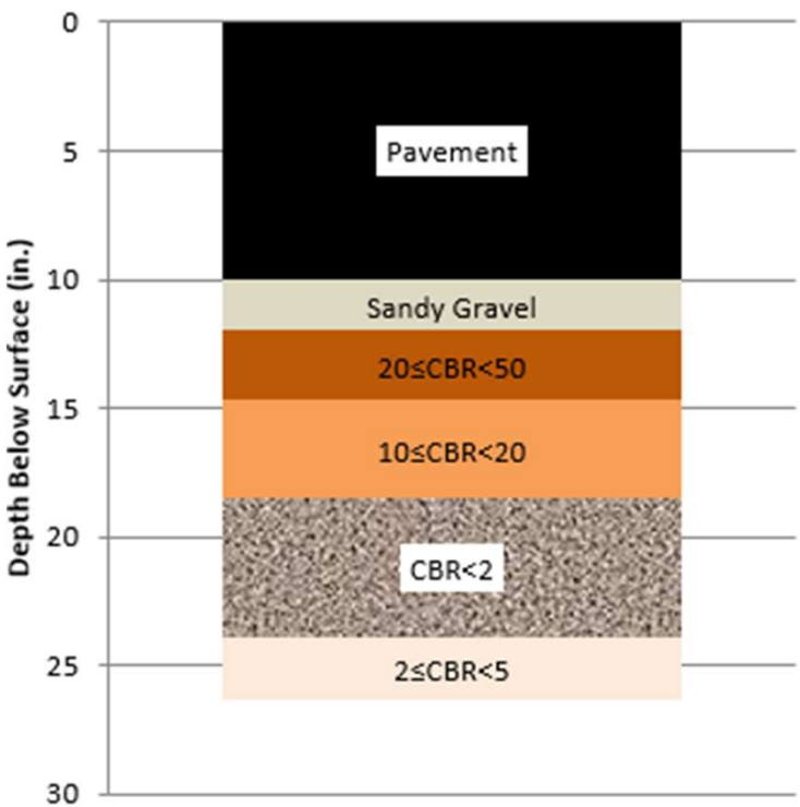
CBR vs. Depth Below Surface (in.) Location #7 - CH 25
