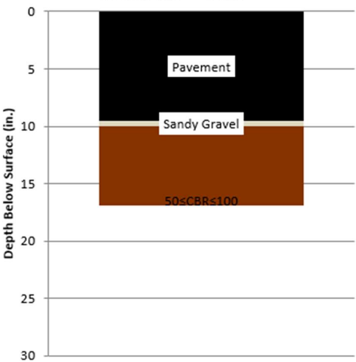
CBR vs. Depth Below Surface (in.) Location #11 - CH 25
