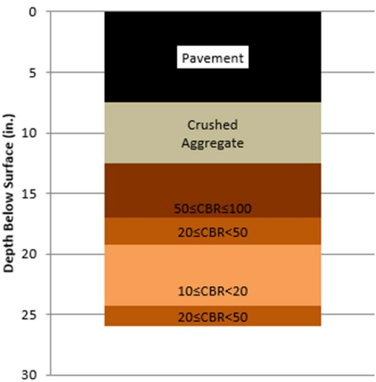
CBR vs. Depth Below Surface (in.) Location #1 - CH 25
