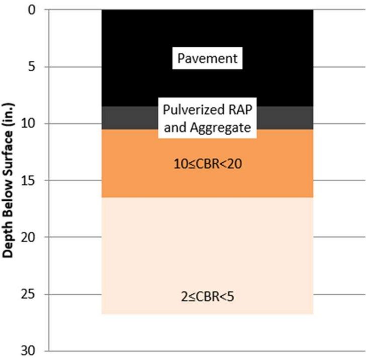
CBR vs. Depth Below Surface (in.) Location #8 - CH 25
