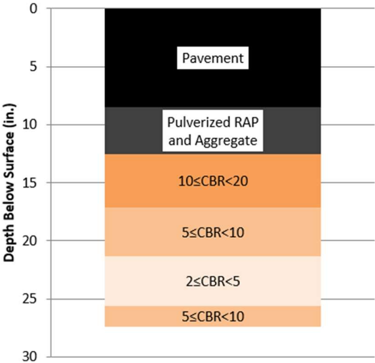
CBR vs. Depth Below Surface (in.) Location #2 - CH 25
