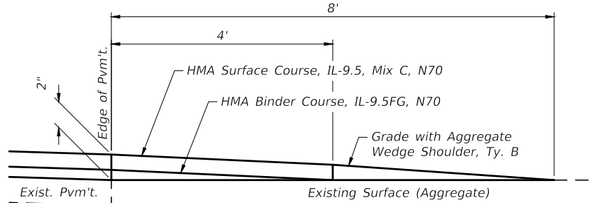
SECTION A-A PRIVATE ENTRANCE - AGGREGATE (Est. No. = 30)
