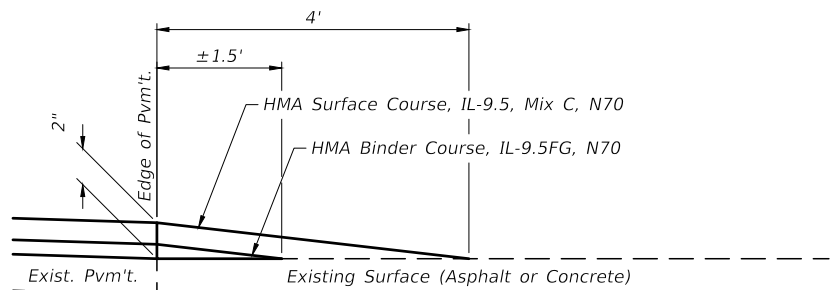
SECTION A-A PRIVATE ENTRANCE - ASPHALT (Est. No. = 1)
