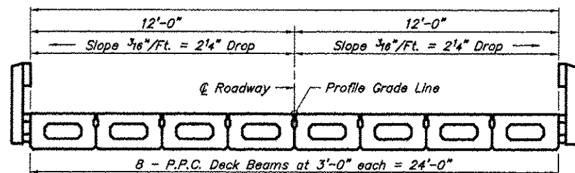
CROSS SECTION
