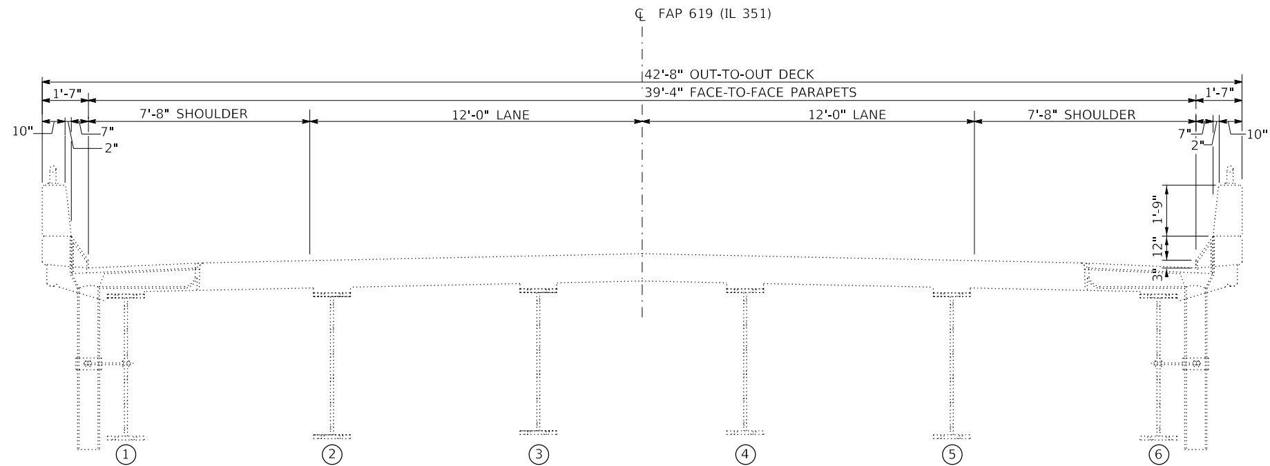
TYPICAL CROSS SECTION STA. 52+64.40 TO STA. 70+38.75
