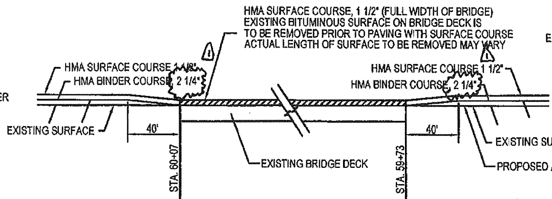
SURFACING AT BRIDGE
