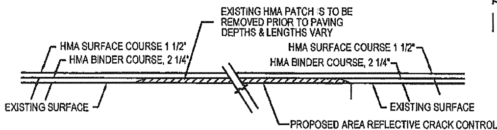
HMA REMOVAL-VARIABLE DEPTH
