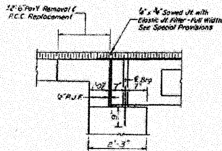
SECTION THRU ABUT NEAR E ROWY
