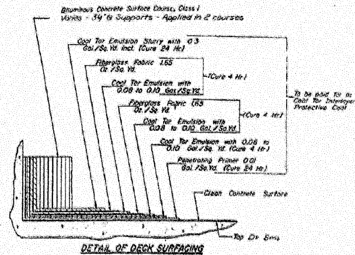
DETAIL OF DECK SURFACING
