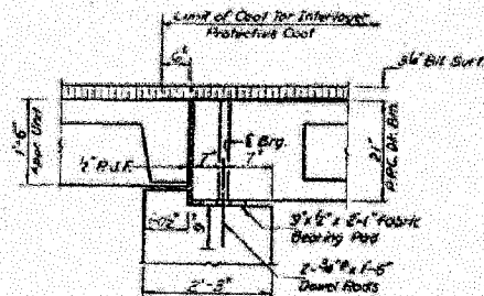
SECTION THRU ABUT AT OUTSIDE BEAM
