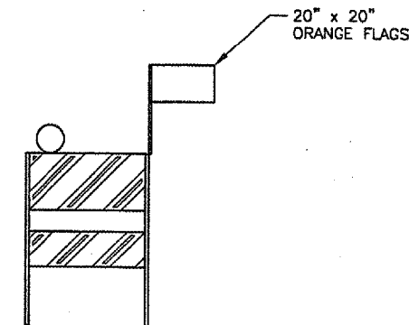
FLASHER BARRICADE DETAIL
