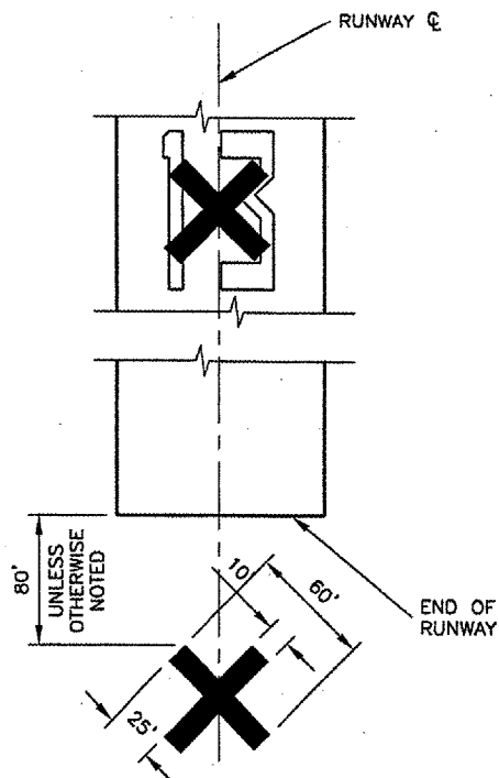
CLOSED RUNWAY MARKER DETAIL
