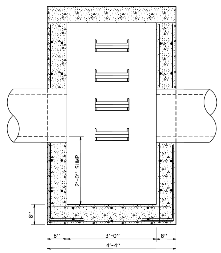
SECTION E-E
