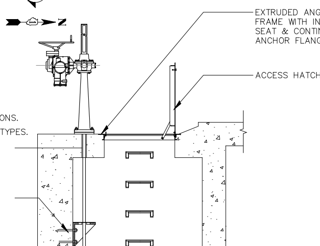
3 ACCESS HATCH DETAIL SCALE: 1/2" = 1'-0"
