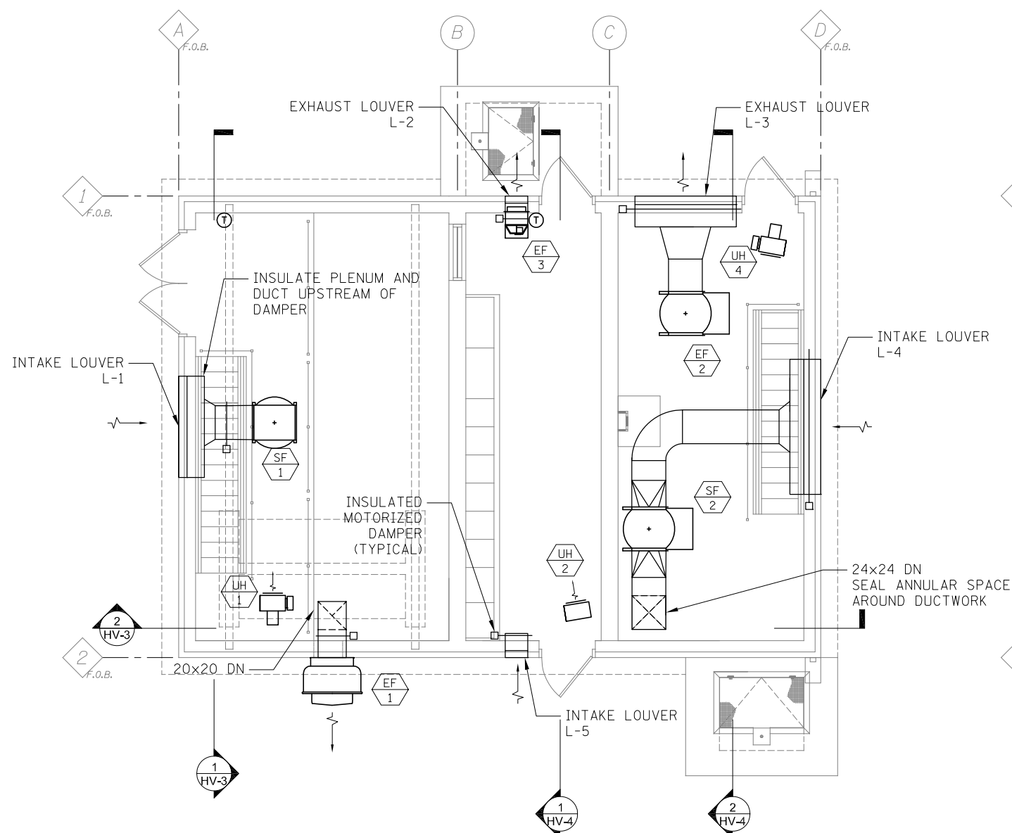
1 GROUND FLOOR PLAN - EL: 701.50 SCALE: 1/4" = 1'-0"
