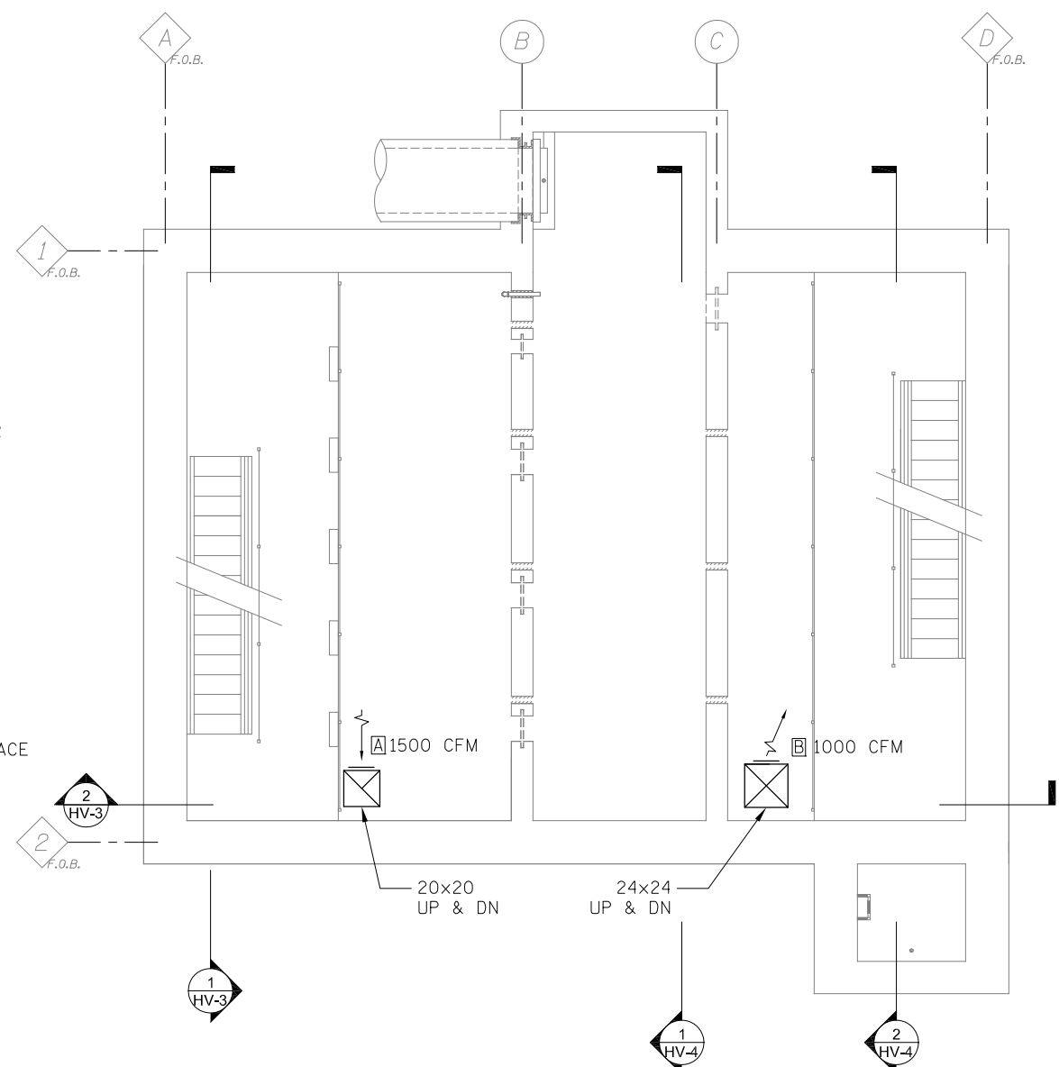
2 INTERMEDIATE FLOOR PLAN (-1) - EL: 692.75 SCALE: 1/4" = 1'-0" - DISCHARGE EL: 694.00 HP
