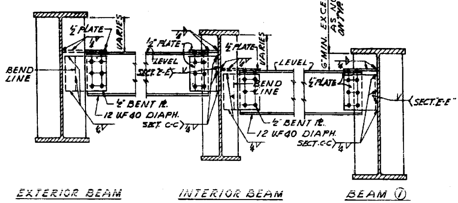
SECTION C-C SHOWN SECTION E-E SIMILAR
