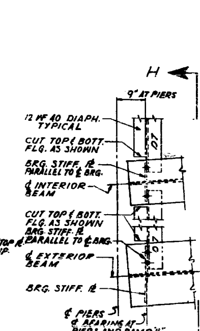
DETAIL #8 PIER #9 SHOWN, PIER #10 AND RAMP #11 SIMILAR
