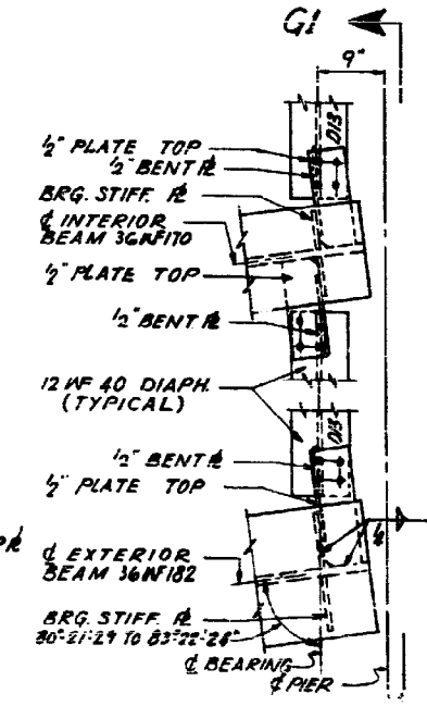
DETAIL #7 PIER #6 & #8 SIMILAR
