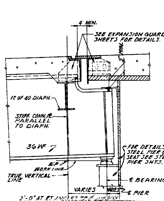
VIEW V-V
