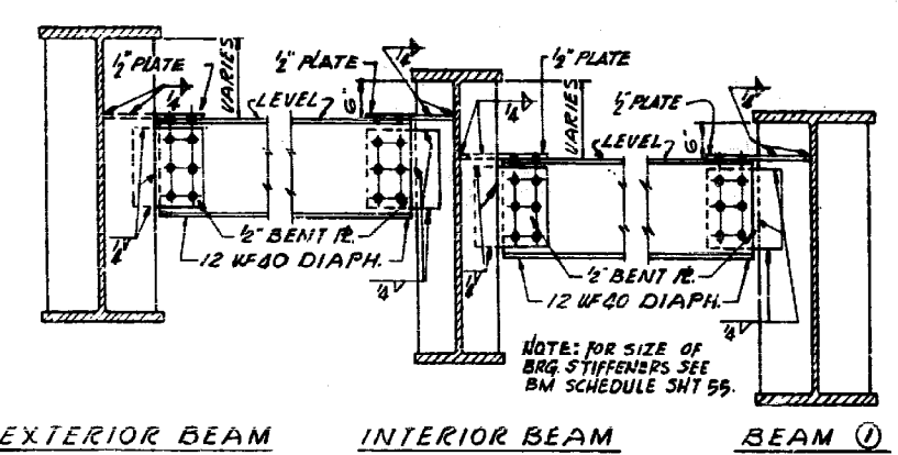
SECTION G-G SECTION G1-G1 SIMILAR
