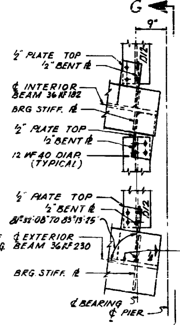
DETAIL #6 PIER #3 SHOWN PIER #2 SIMILAR
