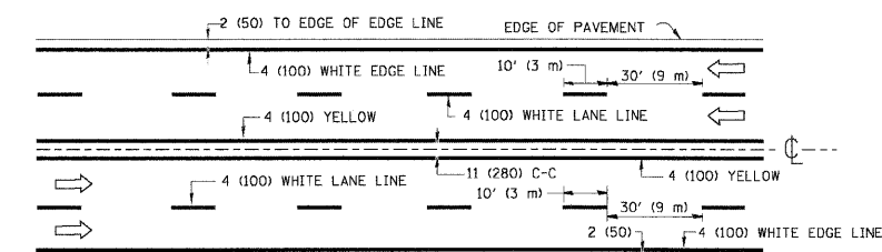
MULTI-LANE UNDIVIDED
