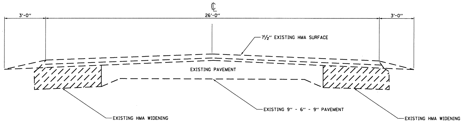
TYPICAL SECTION
