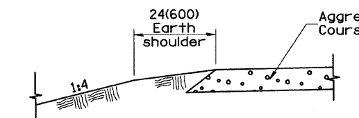
SECTION A-A SHOULDER TREATMENT FOR AGGREGATE ENTRANCES
