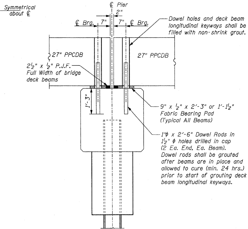
FIXED BEARING PIER
