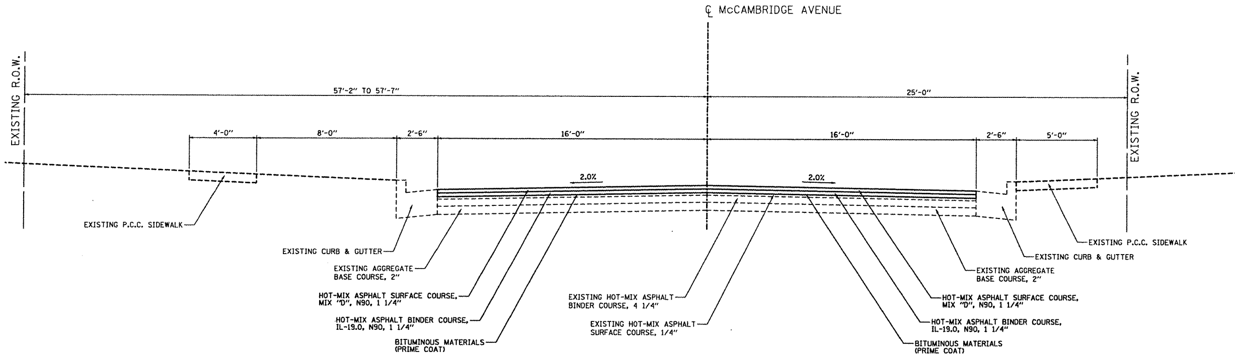
McCAMBRIDGE AVENUE PROPOSED TYPICAL SECTION STA. 212+98.43 TO STA. 215+79.14 (NOT TO SCALE)
