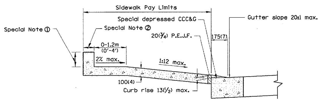
SEC. C-C
