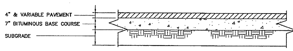
AREA D EXISTING TYPICAL SECTION NTS
