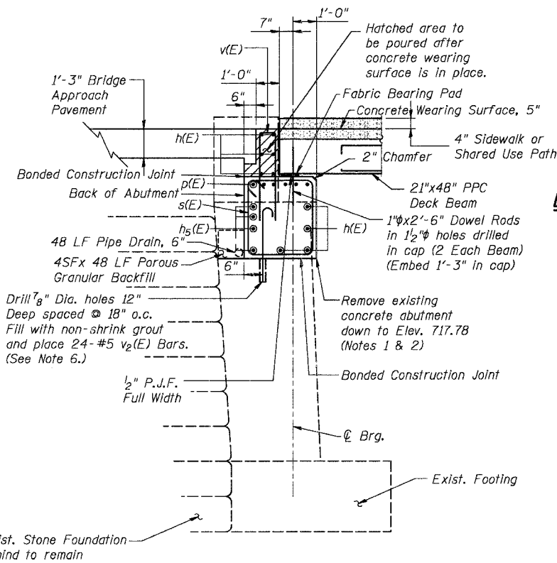
SECTION THRU ABUTMENT (Looking North) Not To Scale
