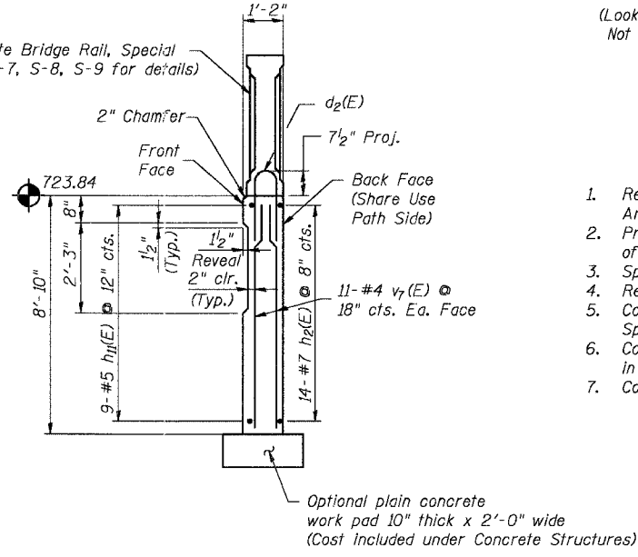
SECTION A-A Not To Scale (See S-10)
