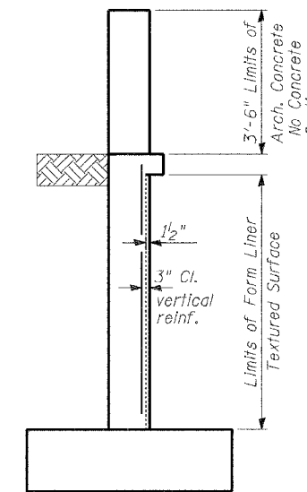
SECTION THRU RETAINING WALLS
