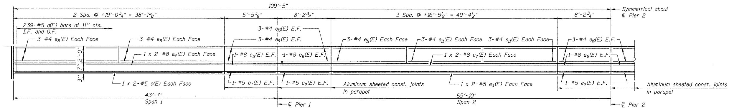
INSIDE ELEVATION MEDIAN BARRIER
