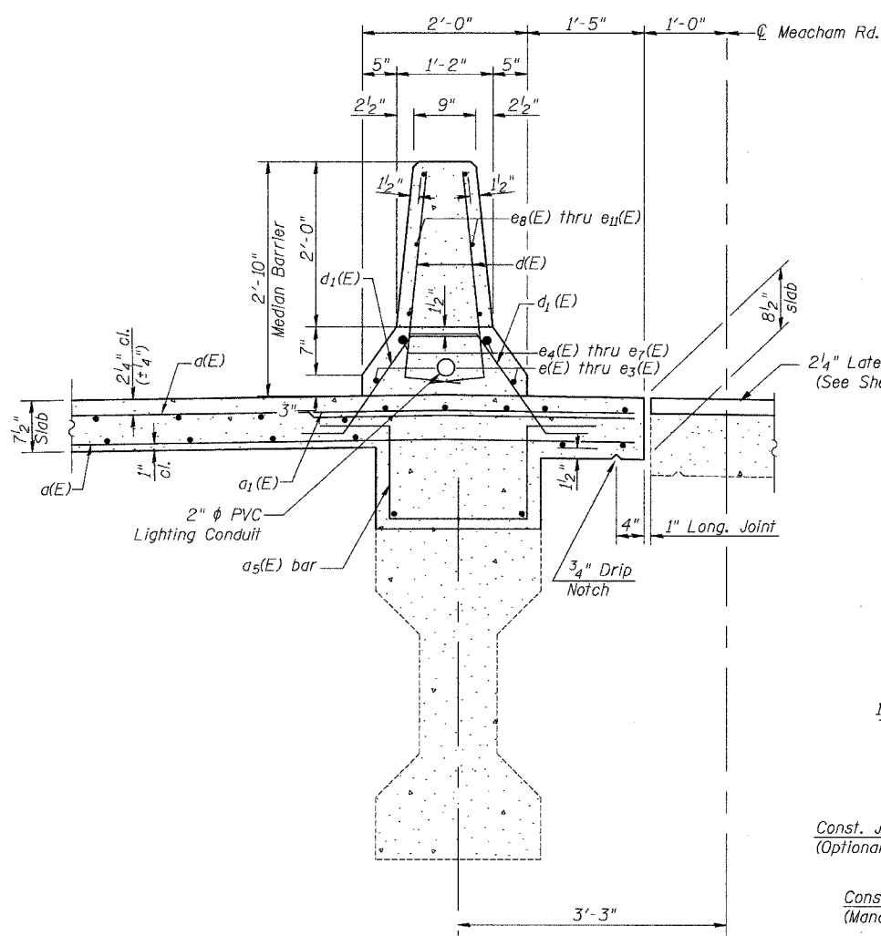
SECTION THRU MEDIAN BARRIER
