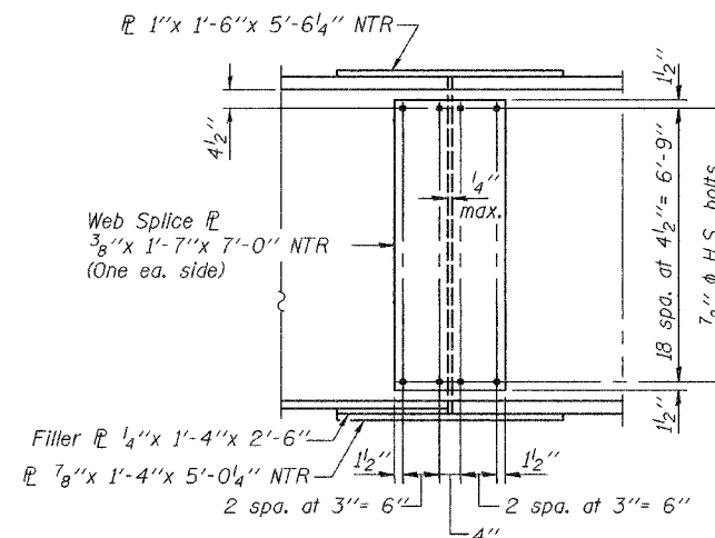
ELEVATION - SPLICE 5
