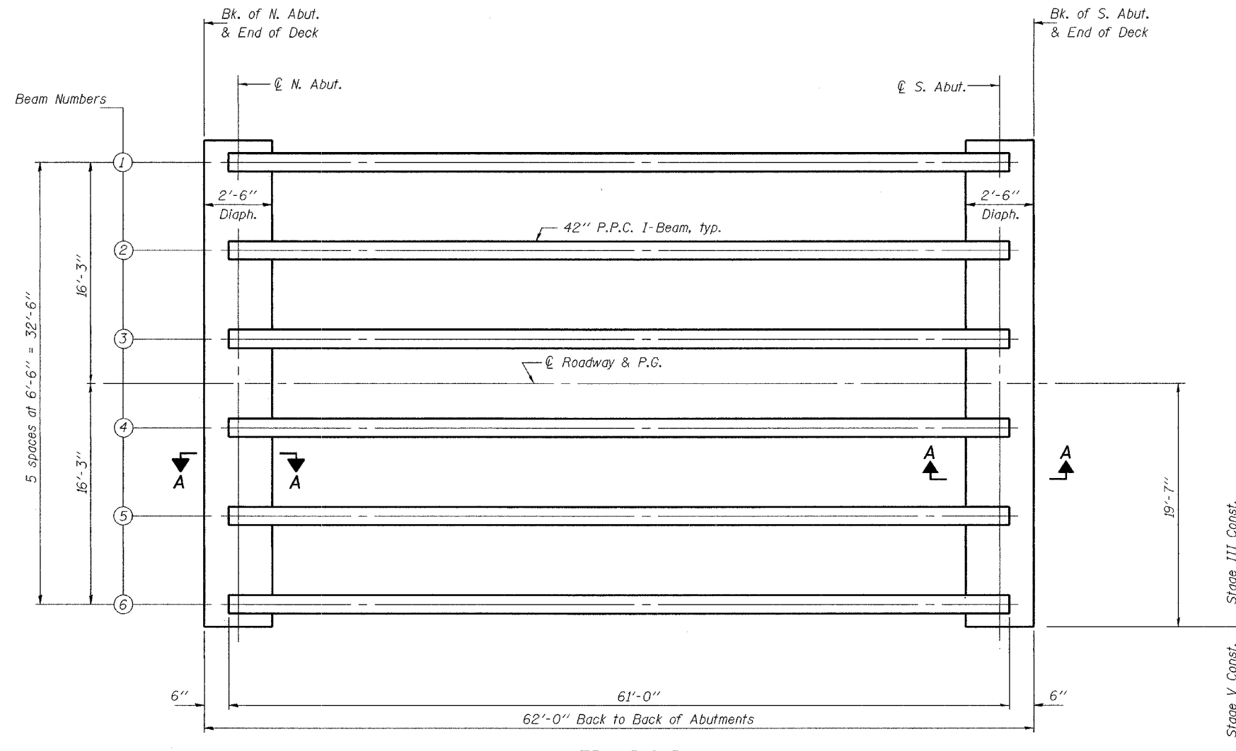
FRAMING PLAN
