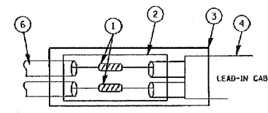
DETAIL "B" LOOP-TO-CONTROLLER SPLICE
