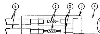
DETAIL "B" LOOP-TO-CONTROLLER SPLICE
