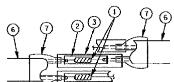
DETAIL "A" LOOP-TO-LOOP SPLICE
