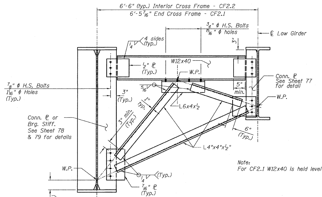
END CROSS FRAME CF2.1
