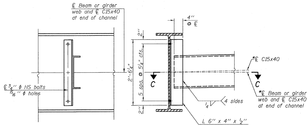
INTERIOR DIAPHRAGM
