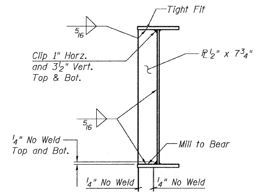
CONN. P DETAILS (FB-4.8, FB-4.9, FB-4.12)
