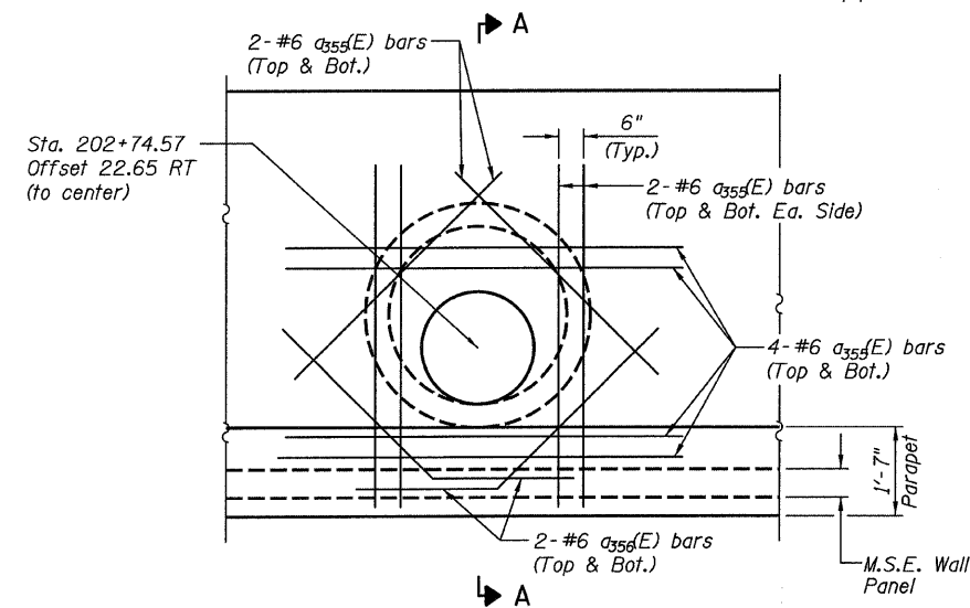
PLAN AT CATCH BASIN
