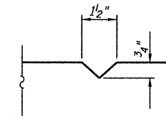
CONTROL JOINT DETAIL - PARAPET
