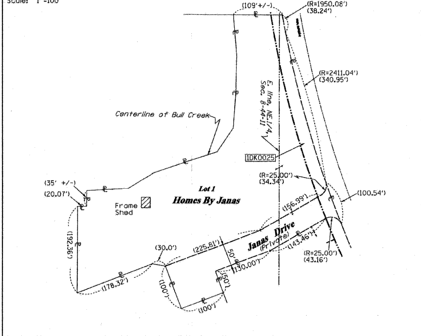
TOTAL HOLDING DIAGRAM PARCEL 1DK0025
