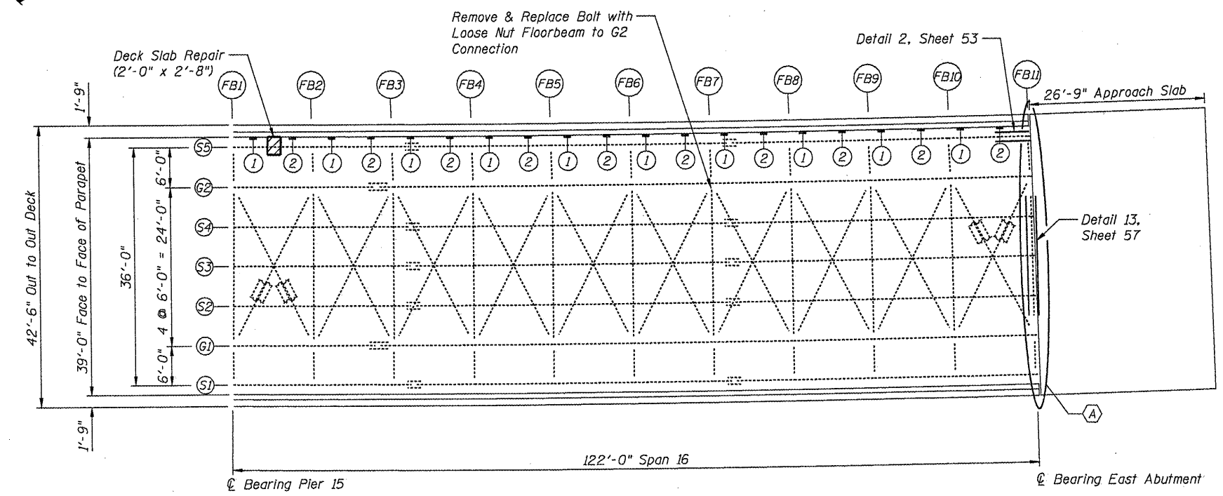
FRAMING PLAN SPAN 16 Eastbound Lanes
