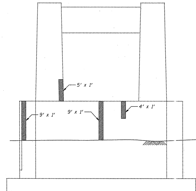
PIER 4 - WEST ELEVATION
