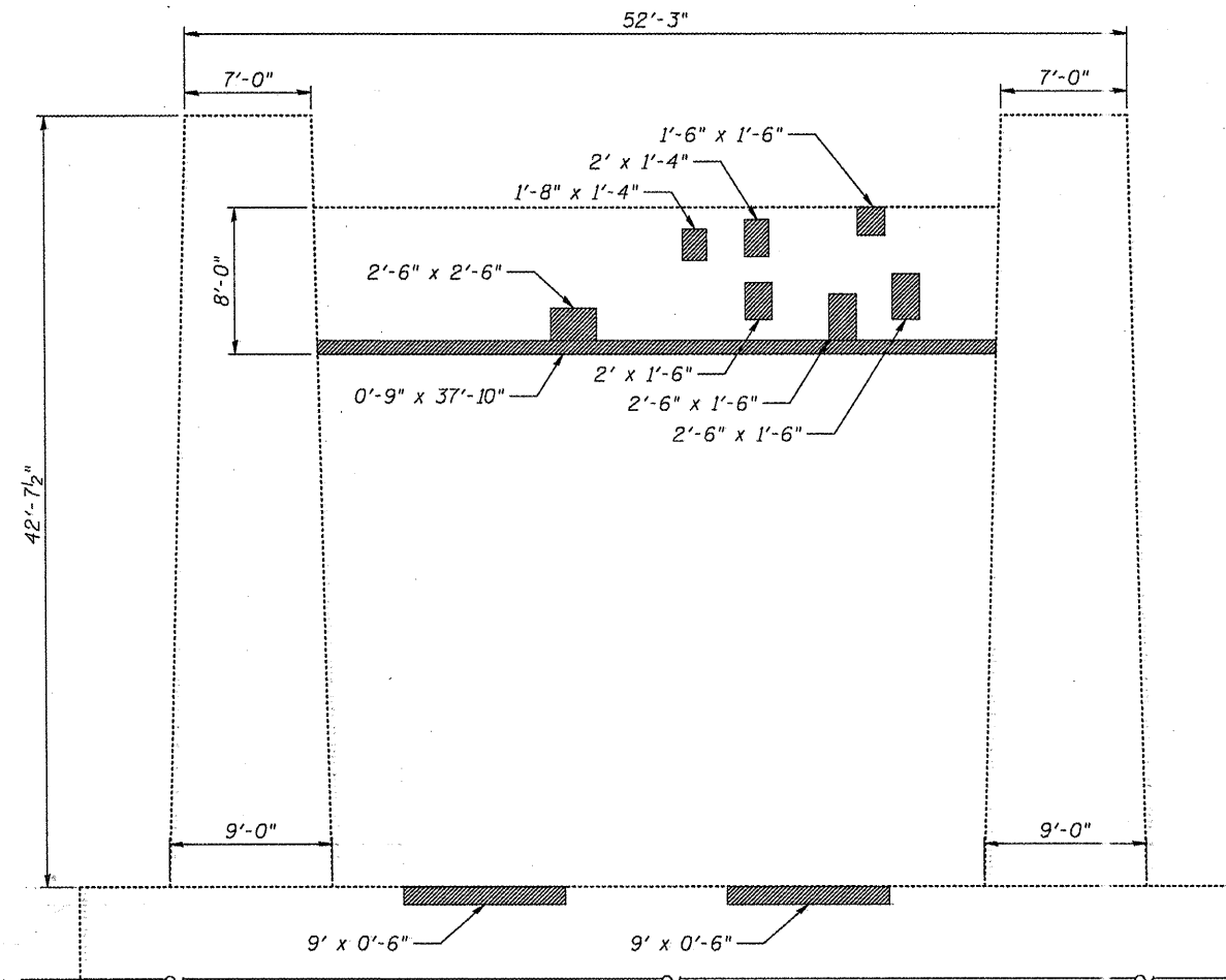
PIER 8 - WEST ELEVATION (Dimensions taken from existing drawings)
