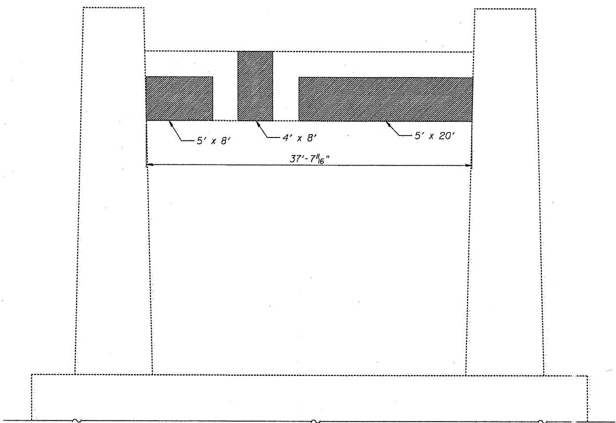
PIER II - WEST ELEVATION (Dimensions taken from existing drawings)
