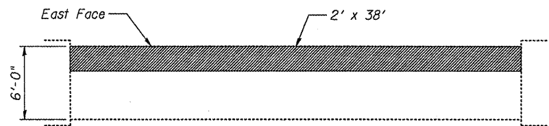
TIE BEAM UNDERSIDE PLAN
