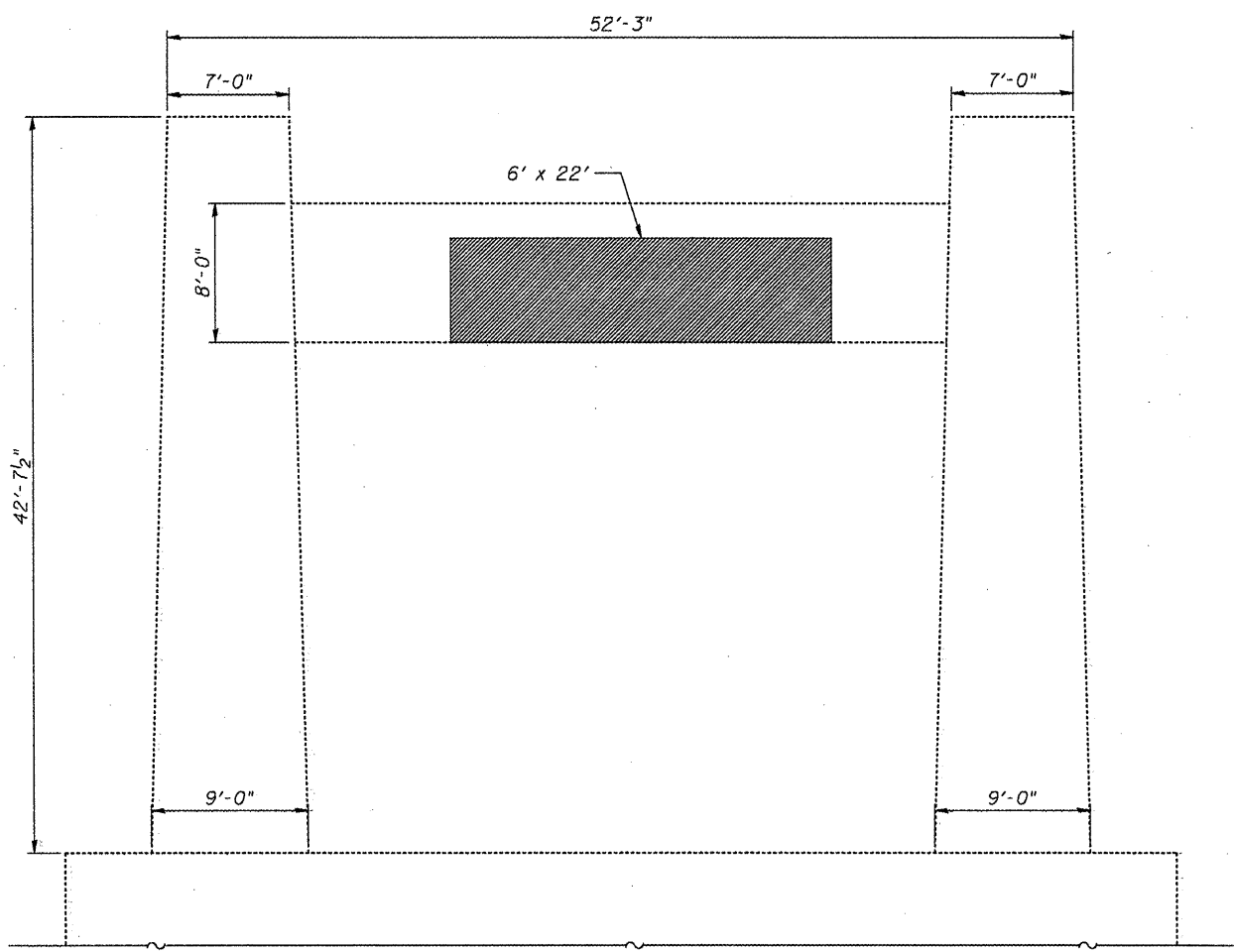
PIER II - EAST ELEVATION (Dimensions taken from existing drawings)
