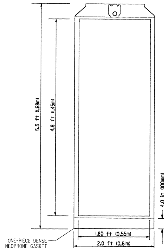
FRONT VIEW (DOOR REMOVED) (MODEL 334)
