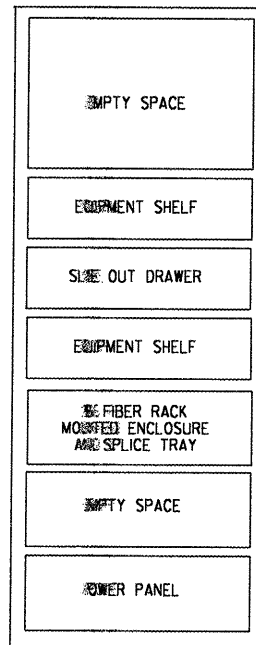
CONTROL CABINET LAYOUT (TYPICAL) (MODEL 334)
