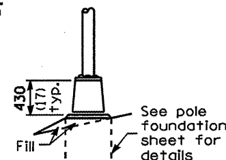
TRANSFORMER BASE
