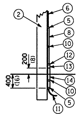
POLE, WOOD
