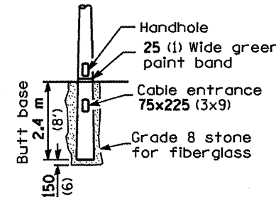
BUTT BASE
