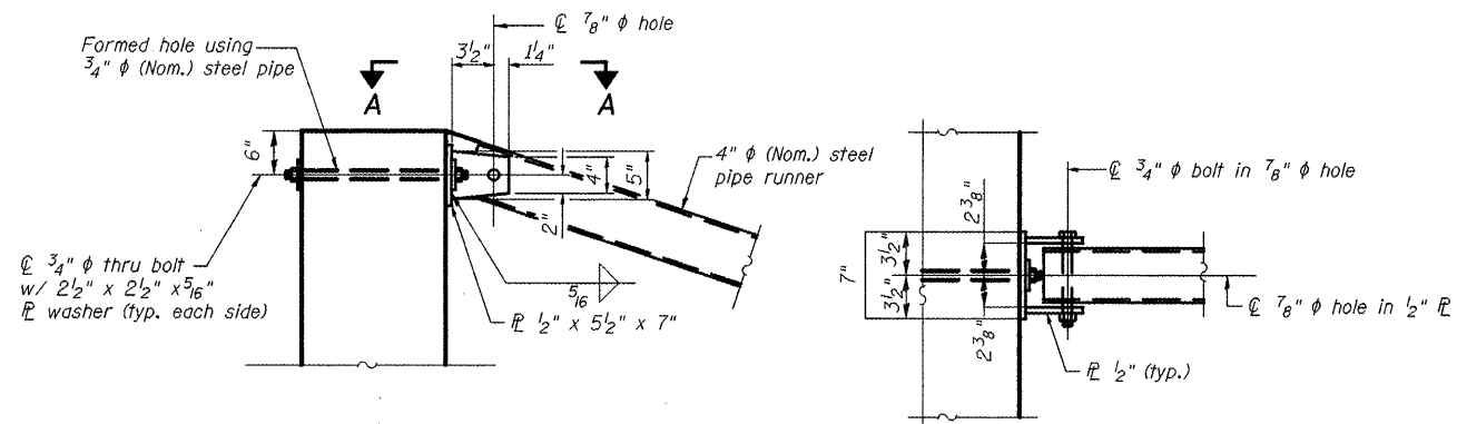
DETAIL A
